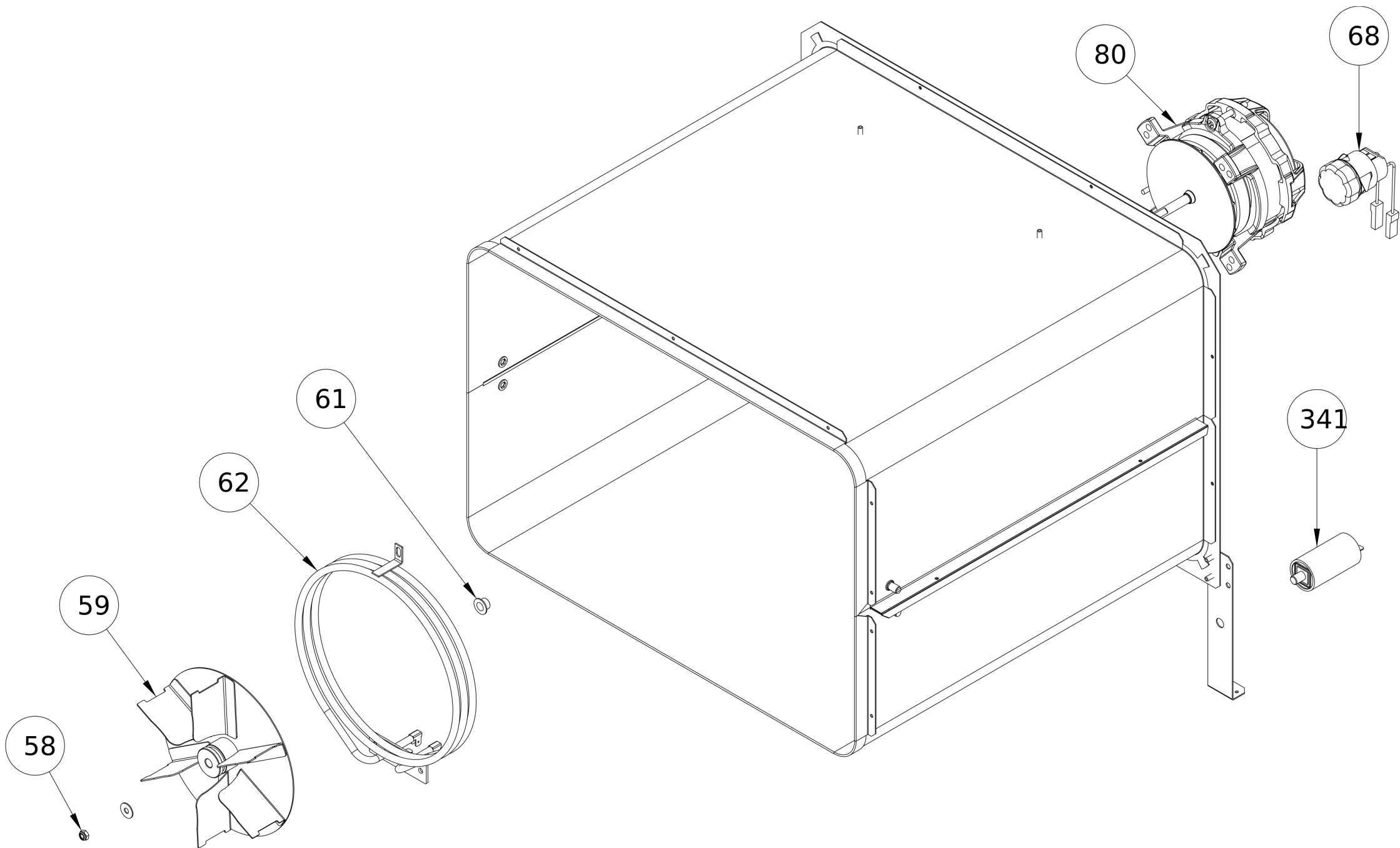
Cooking chamber
