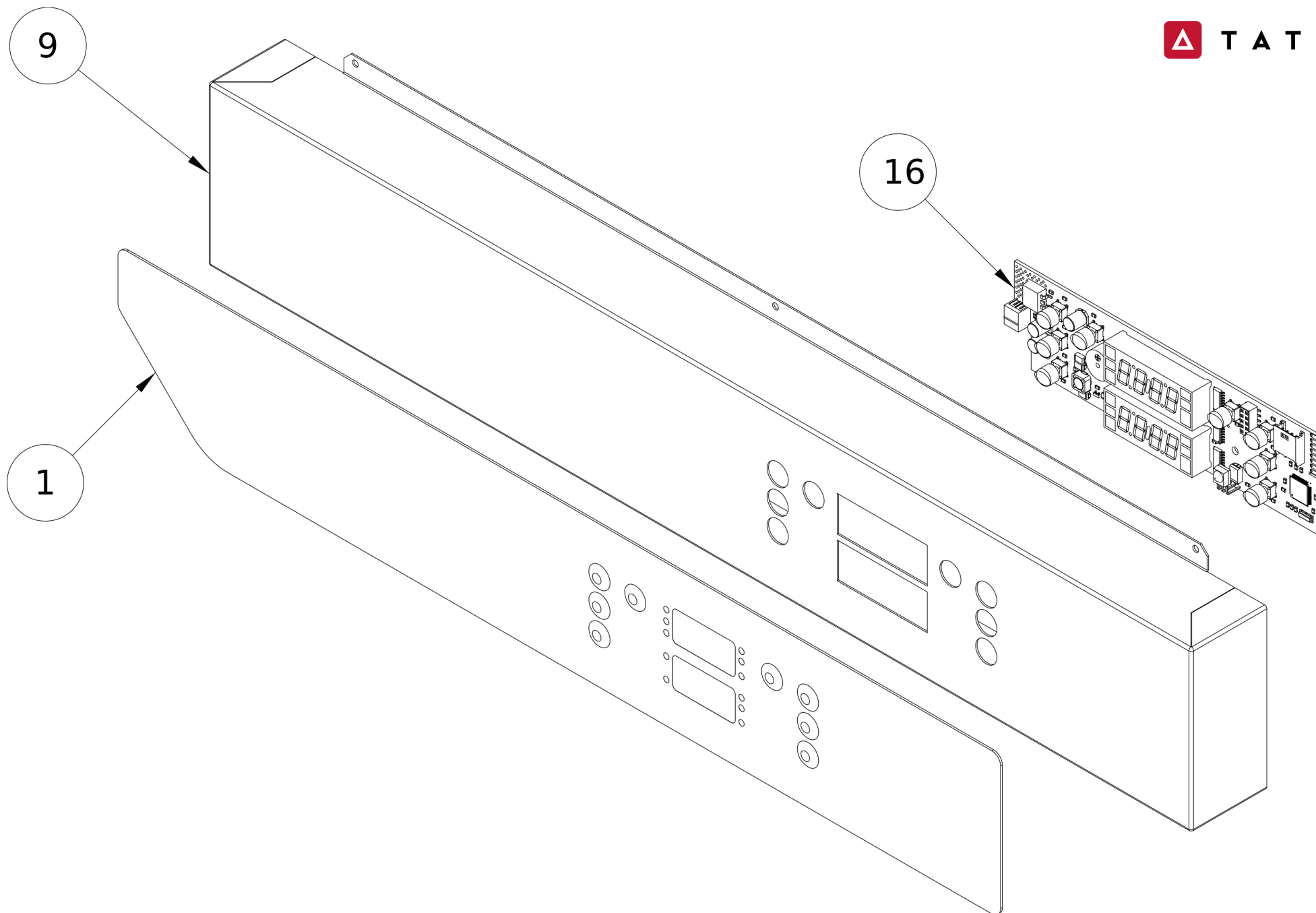
Frontal panel
