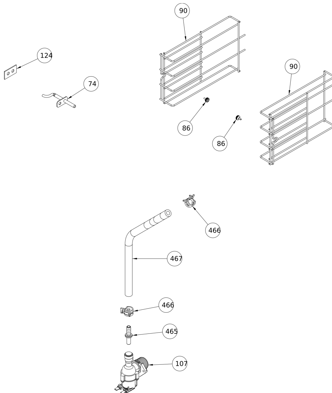
Internal accessories
