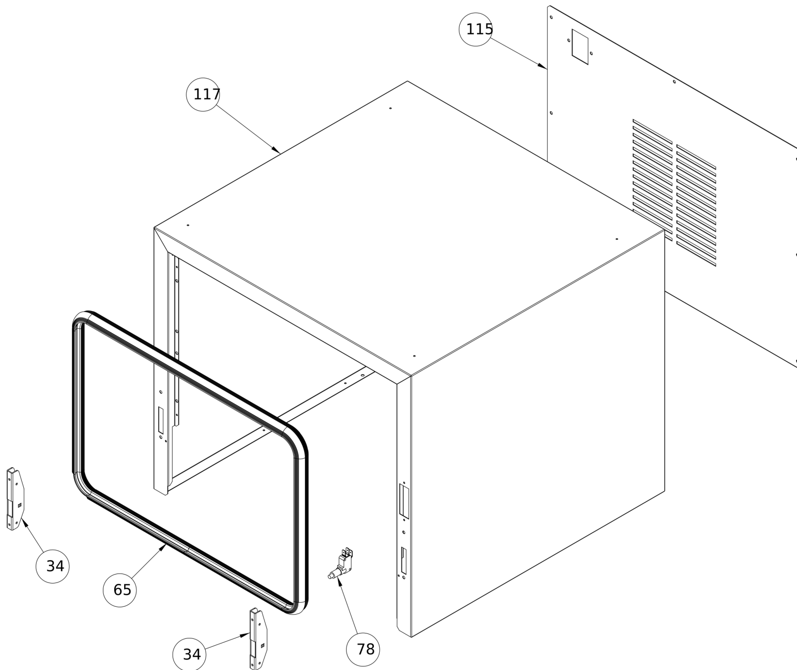
Oven body
