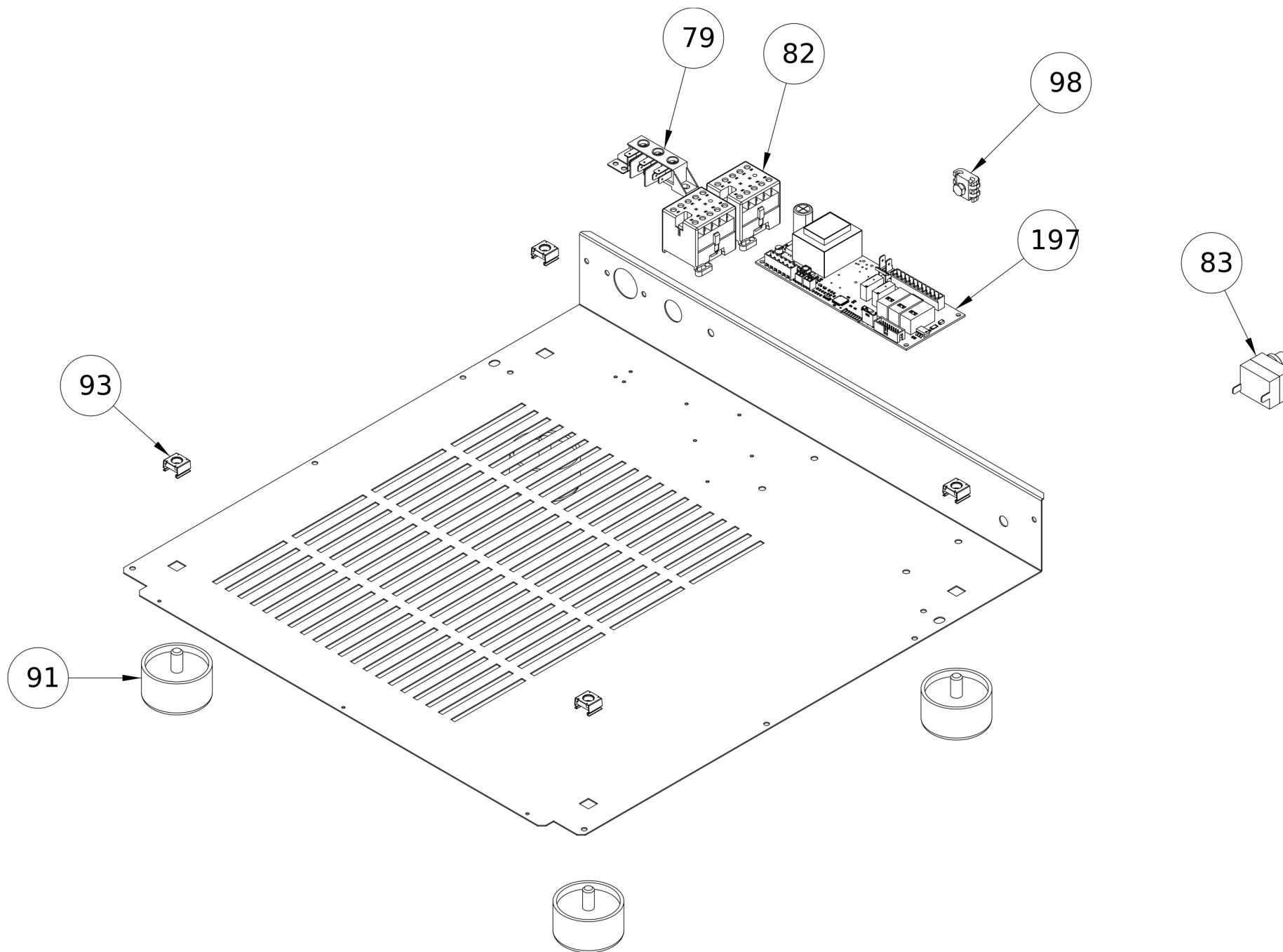
Electrical box
