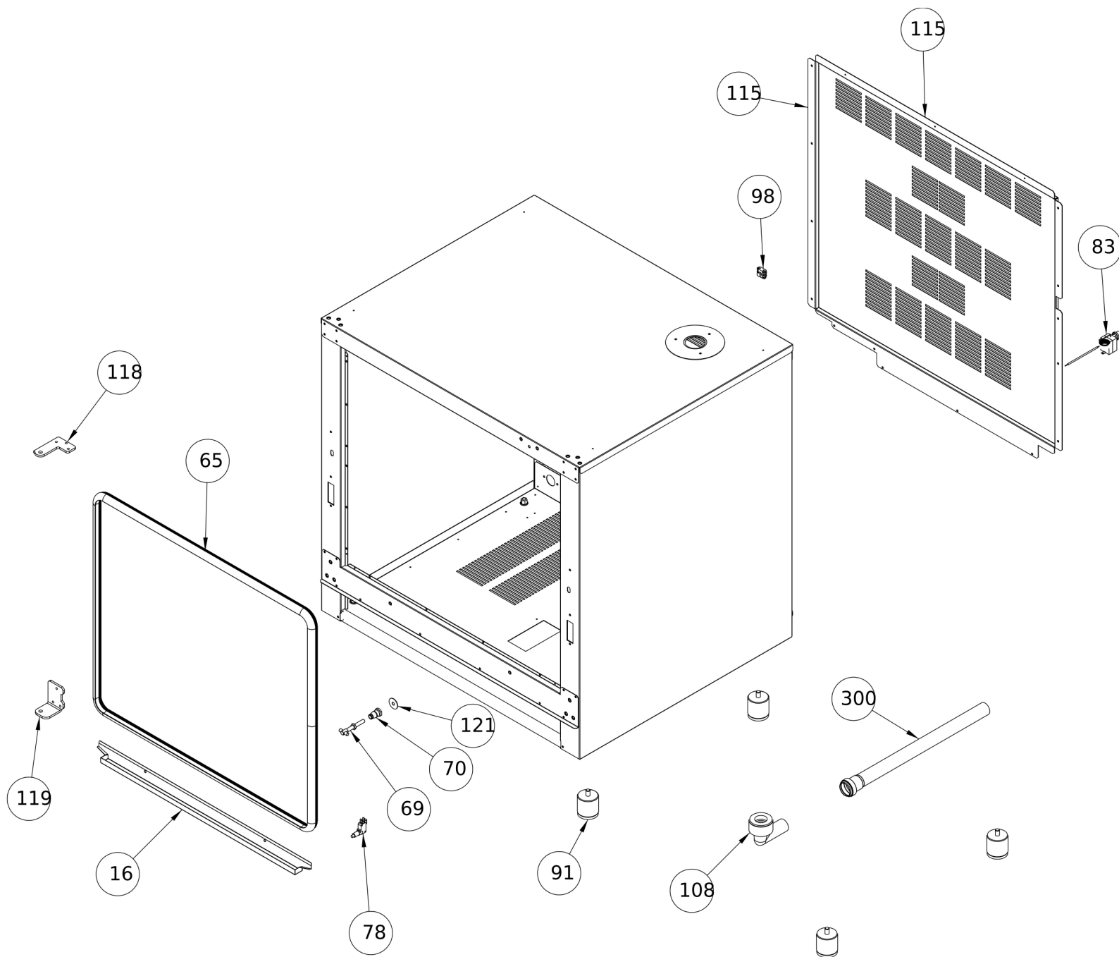
Oven body
