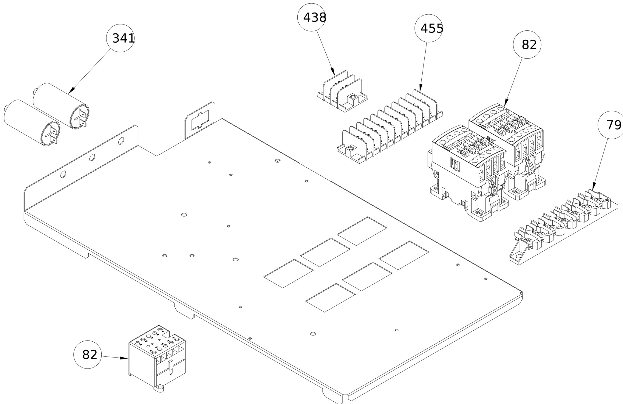
Electrical box
